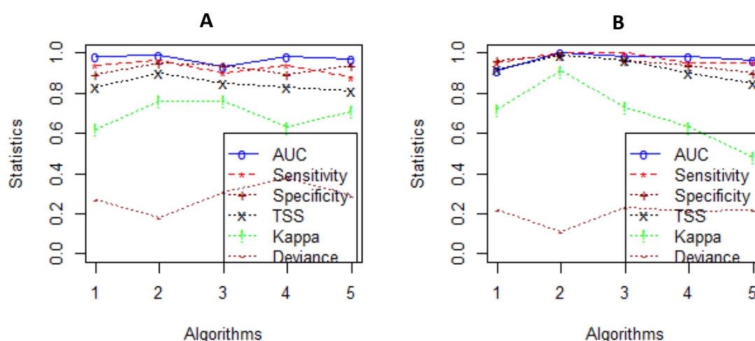
Figure 4: Performance assessment of the five selected algorithms for sugarcane (A) and smooth cayenne (B). 1=Maxent, 2 = Random Forest, 3 = Support-Vector Machines, 4 = Boosted Regression Tree, 5 = Generalized Linear Model
